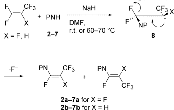
Scheme 1. Addition–elimination reactions of PNH with HFP and PFP, where PNH is the appropriate pyrimidine 2–5 or purine 6 or 7 with endocyclic N 1 for pyrimidines and endocyclic N 9 for purines.
