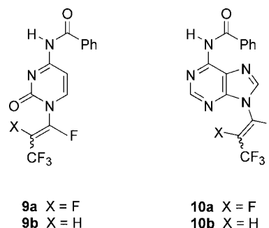
Figure 4. Fluorinated enamines of adenine and cytosine blocked on the exocyclic nitrogen atoms.
