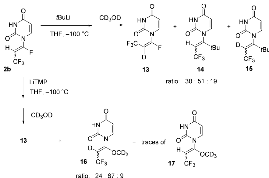
Scheme 4. Different routes for reactions of ( E )- and ( Z )-tetrafluoroprop-1-enyluracil 2b with t BuLi and LiTMP.
