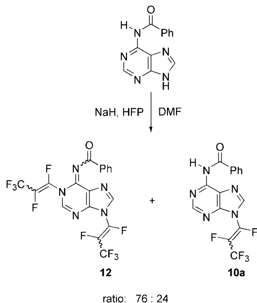
Scheme 3. The reaction between compound 10 and HFP in the presence of a fourfold excess of NaH.
