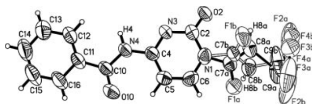
Figure 5. The molecule of ( Z )- 9b viewed in perpendicular to its average plane. Two positions of the tetrafluoropropenyl substituent have been indicated, one with the full and the other with open bonds. The thermal ellipsoids are indicated at the 50% probability level.
