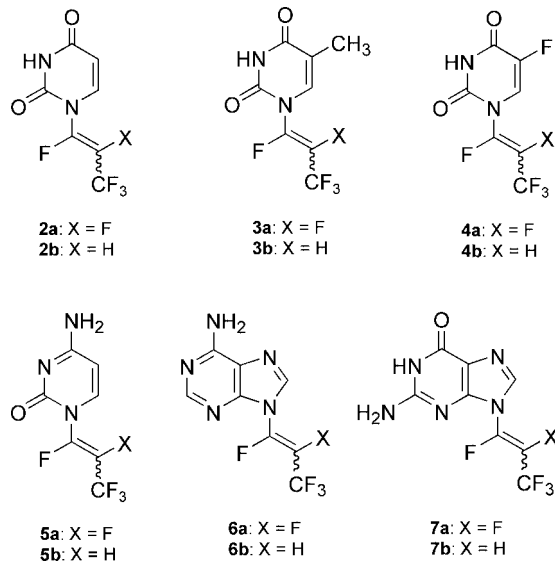
Figure 2. Fluorinated enamines of nucleobases.
