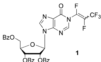
Figure 1. N 1 -(Perfluoroprop-1-enyl) derivative of tribenzoylinosine.
