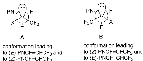
Figure 3. Two possible transition states of carbanion 8 .
